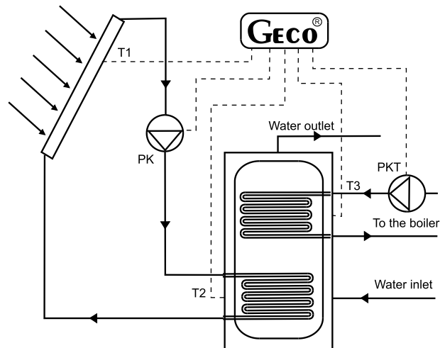
Rys. 2 System with one solar collector and boiler pump.
