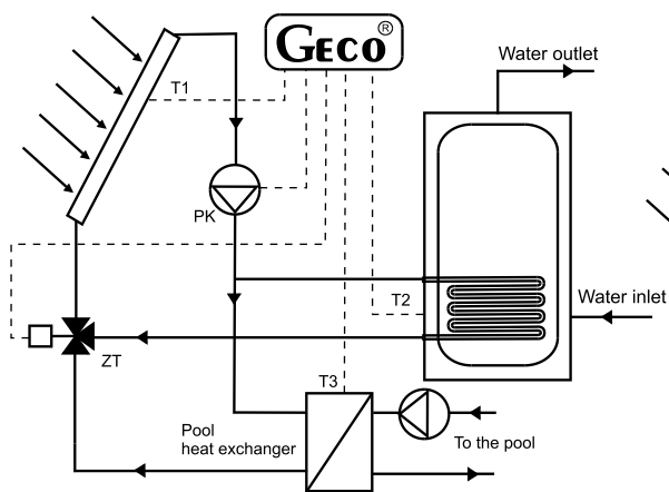
Rys.4 System with one solar collector and pool heating
