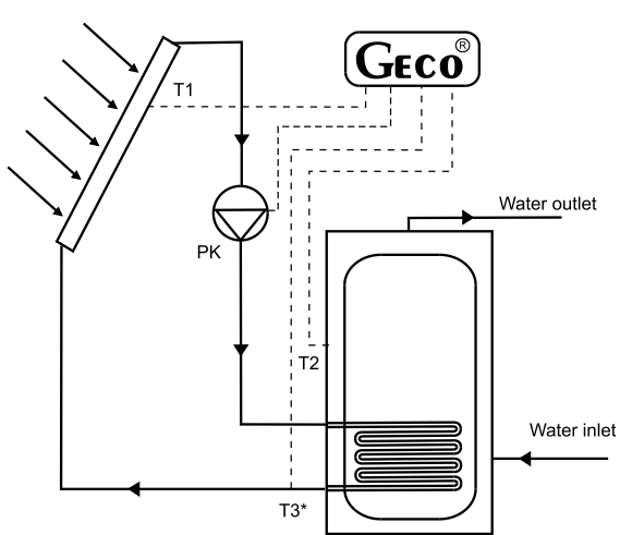
Rys. 1 Basic system with one collector
