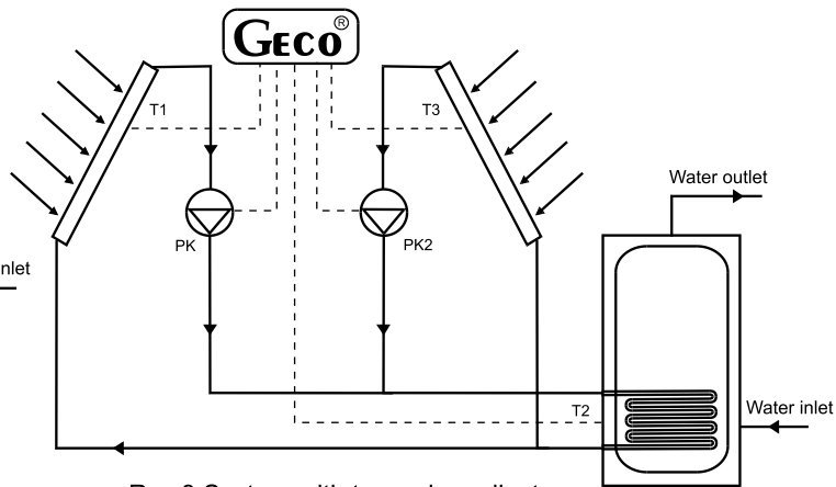
Rys.3 System with two solar collectors
