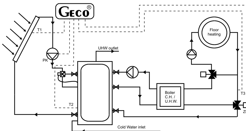
Rys.6 System with one collector and floor heating
