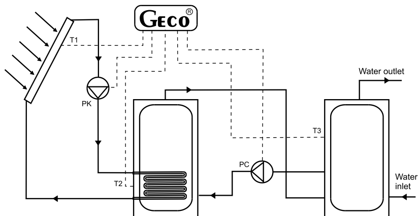
Rys.5 System with one collector and Utility Hot Water pump
