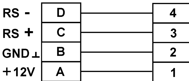
Diagram 12.1 connecting the GA03HA room panel to the GH22RA controller
