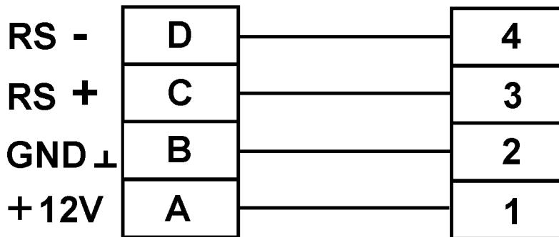
Diagram for connecting the GA03HA room panel to the GH22RA controller
